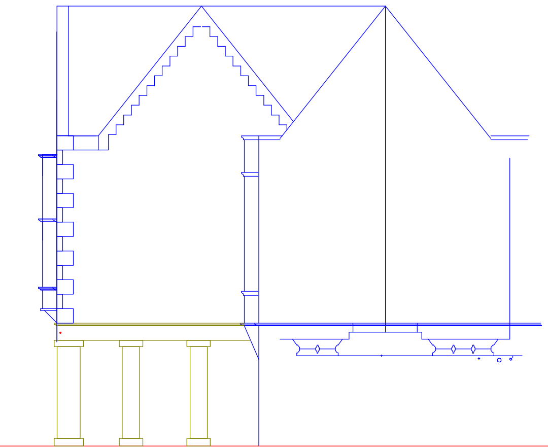
ELEVATION TO NORTH STREET
