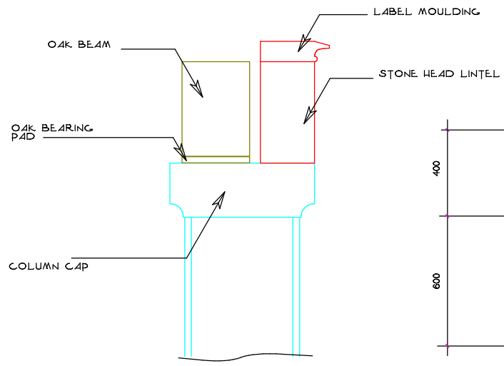
SECTION ON HEAD LINTEL (EXISTING)
