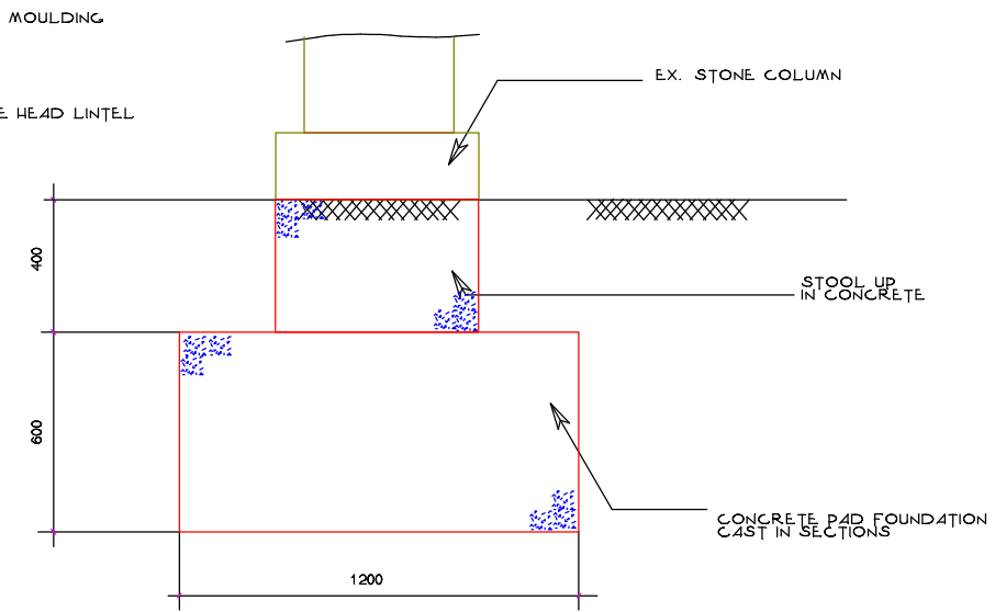
UNDERPINNING DETAIL (EXISTING)
