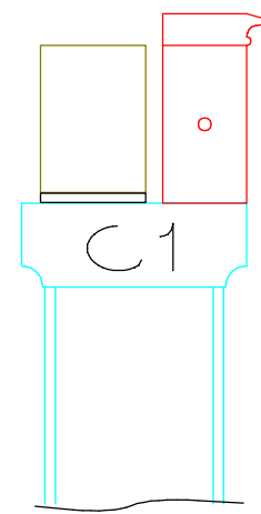
SECTION ON HEAD LINTEL (EXISTING)
